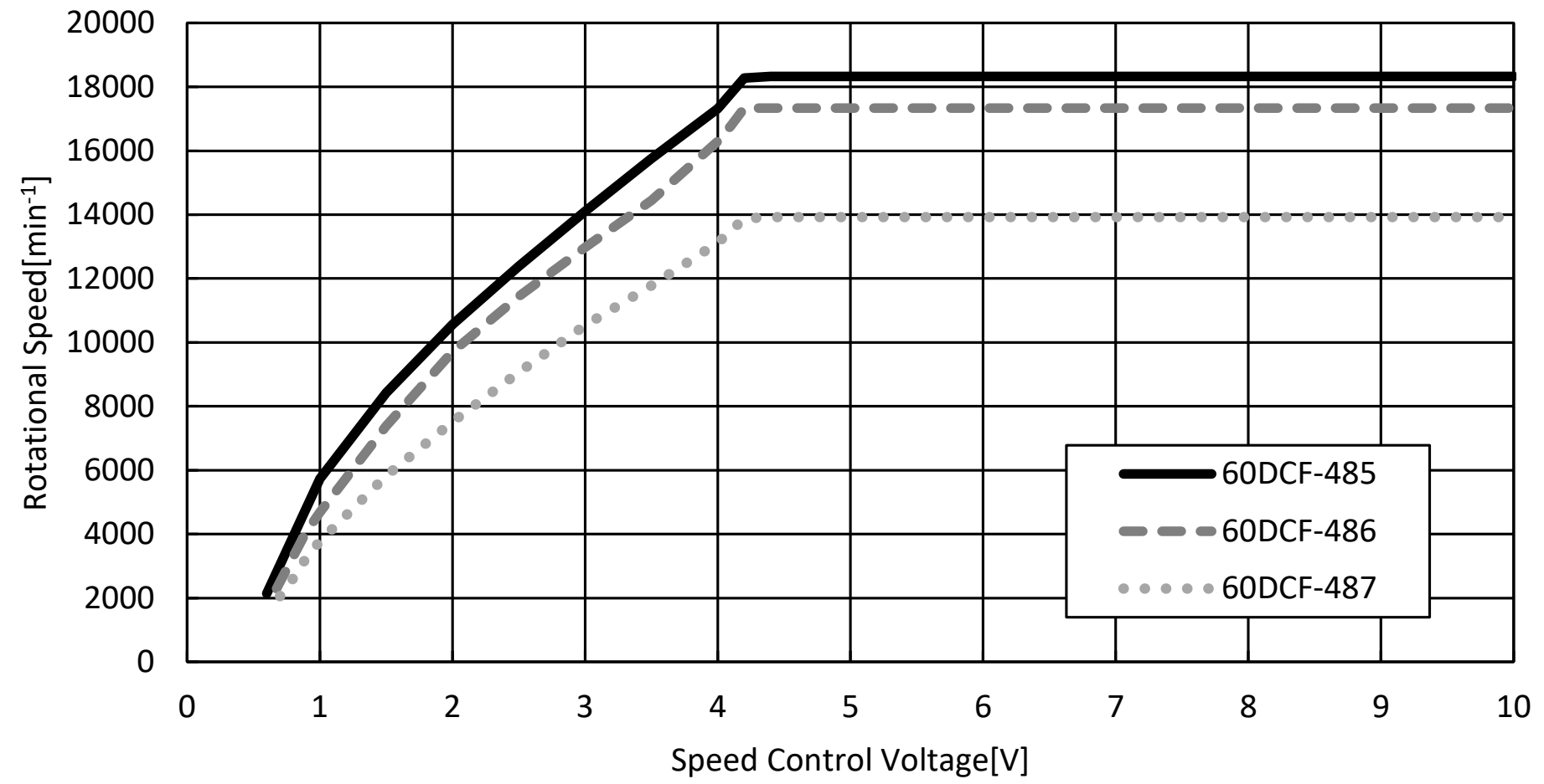
[Reference] Control VS Speed (fully open)
