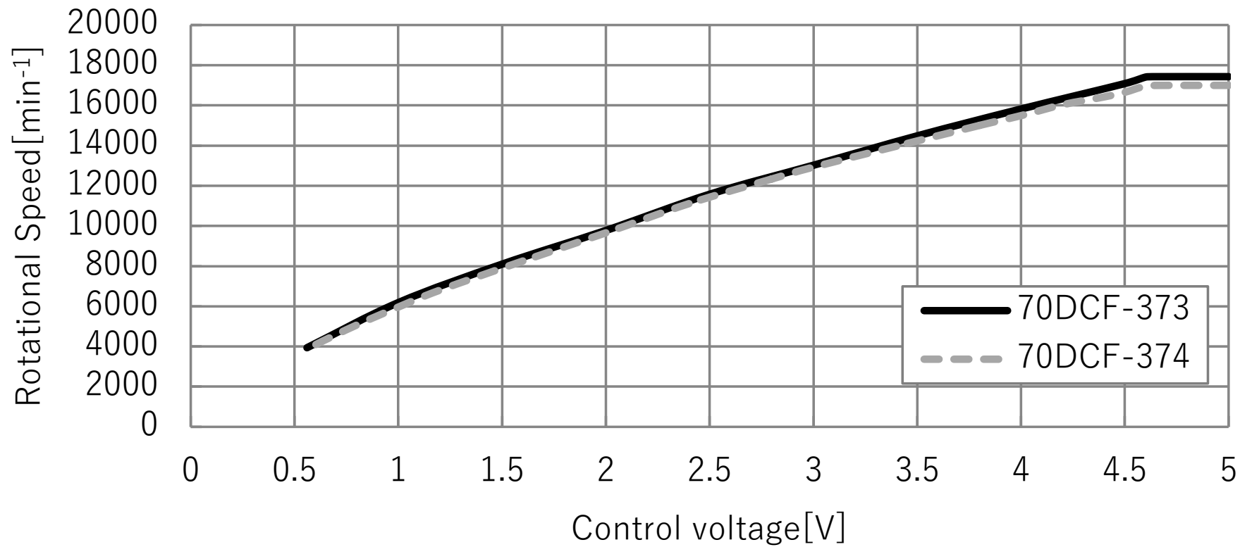
[Reference]Control voltage VS Speed (fully open)
