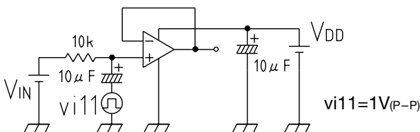
■ Measuring circuit 11
