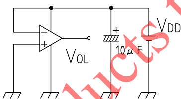
■ Measuring circuit 7
