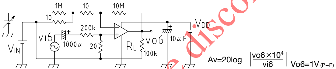
■ Measuring circuit 6
