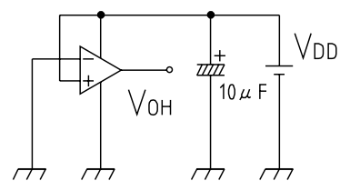
■ Measuring circuit 8
