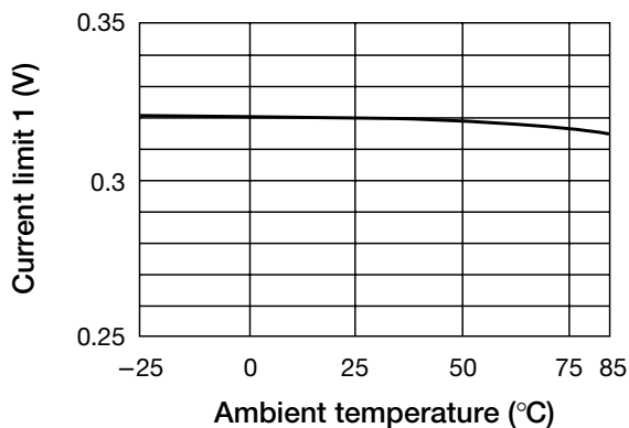
■ Current limit 1 vs Ambient temperature
