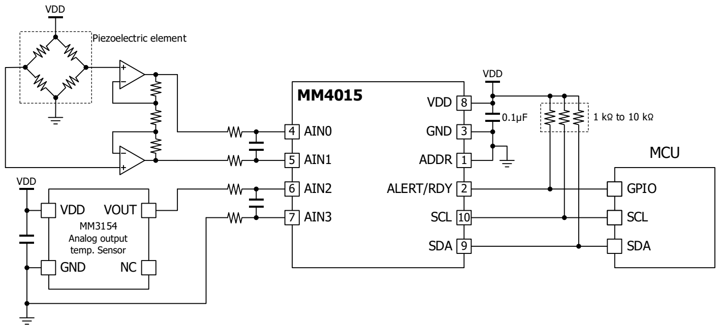
Figure 16. Typical application circuit
