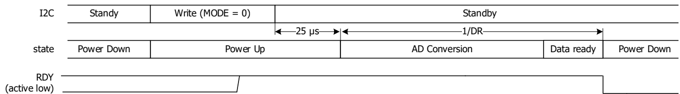
Figure 9. Single-shot conversion
