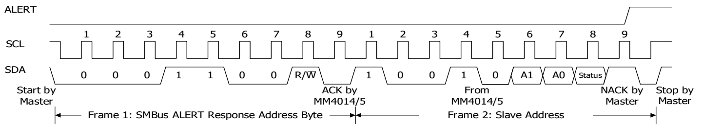
Figure 6. Timing Diagram for SMBus Alert Response
