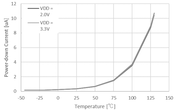
Figure 19. Power-Down Current vs Temperature
