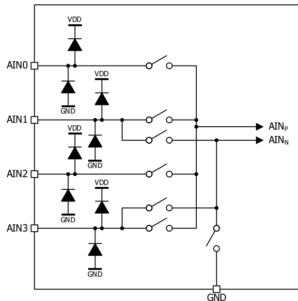
Figure 2. Input Multiplexer
