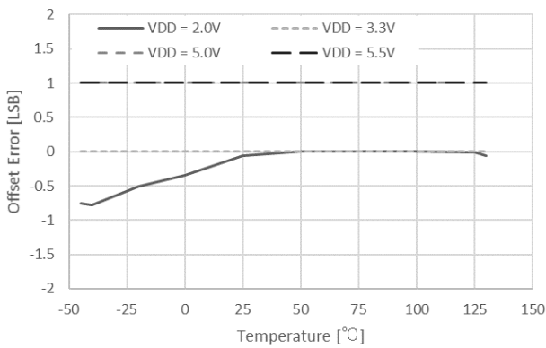
Figure 18. Offset Error vs Temperature
