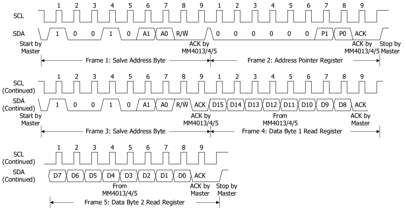
Figure 11. Timing Diagram for Reading from MM4013, MM4014, MM4015
