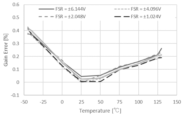
Figure 20. Gain Error vs Temperature
