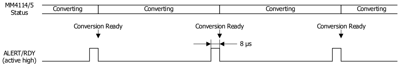
Figure 7. Conversion Ready Pulse in Continuous-Conversion Mode
