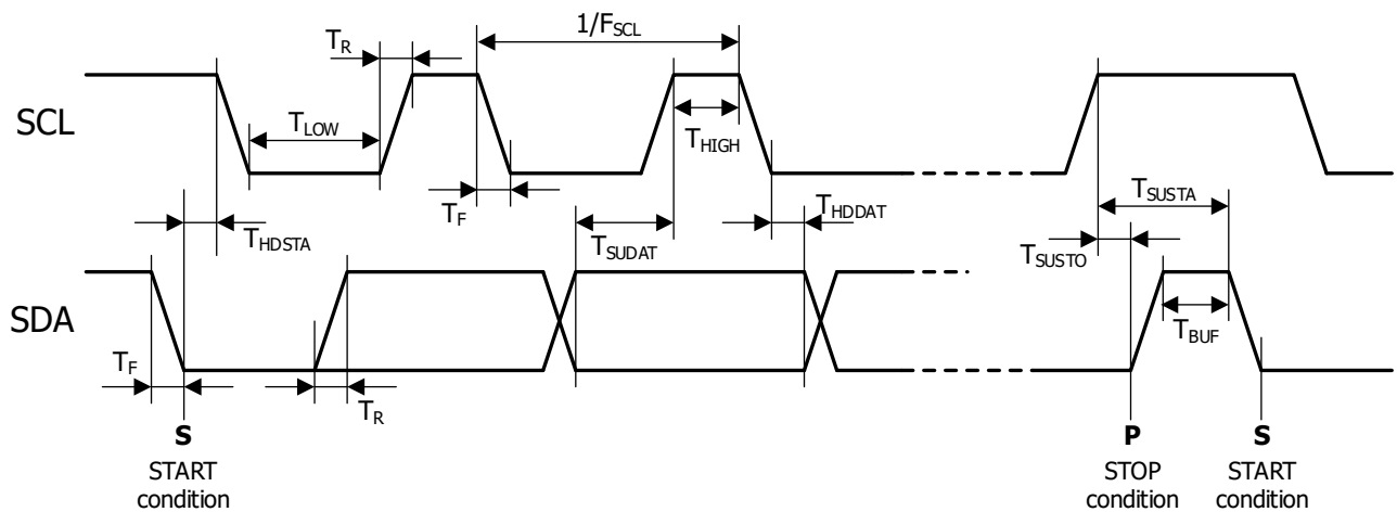
Figure 1. I2C Interface Timing
