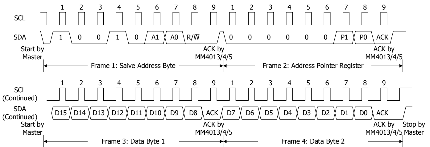
Figure 12. Timing Diagram for Writing to MM4013, MM4014, MM4015
