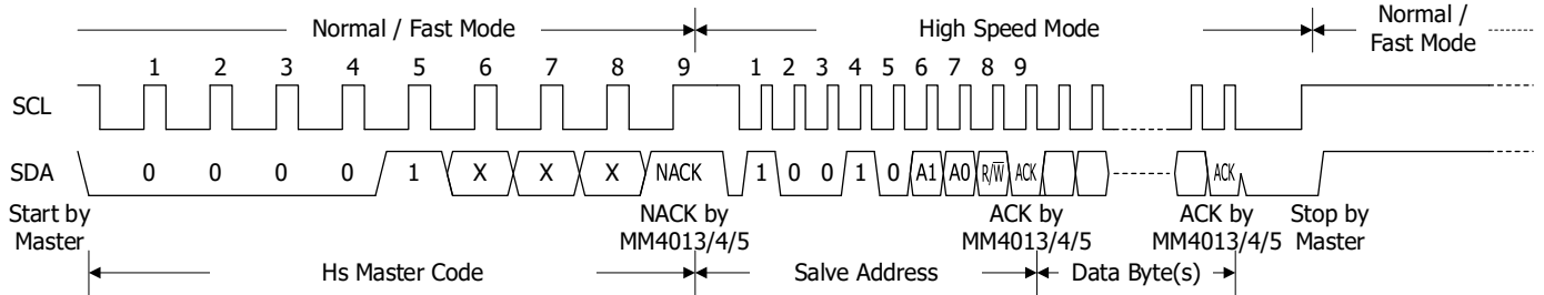
Figure 13. Hs master code
