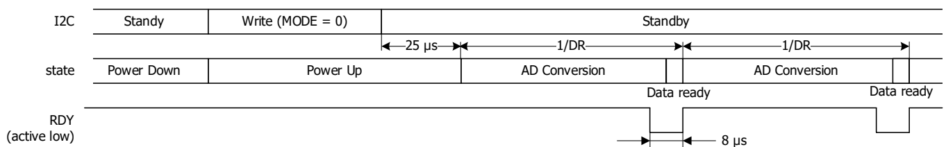
Figure 10. Continuous conversion
