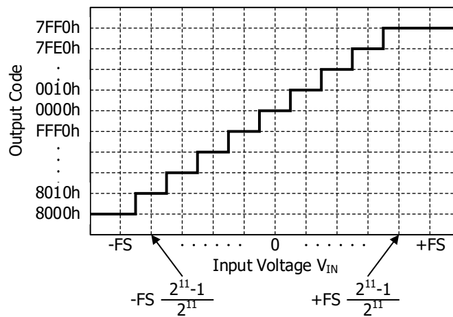
Figure 15. Code Transition Diagram
