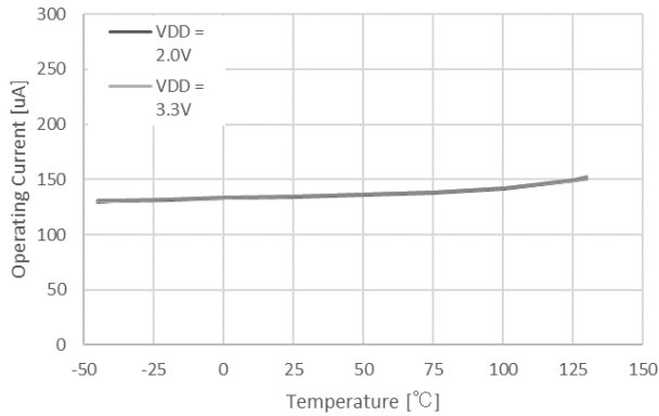
Figure 17. Operating Current vs Temperature
