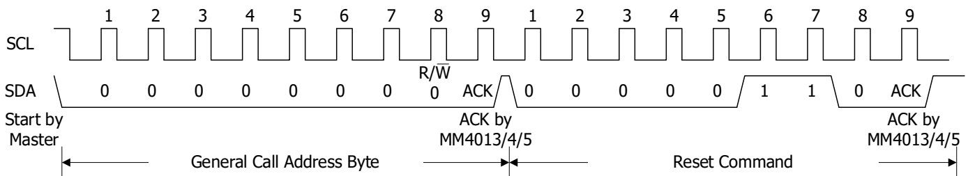
Figure 14. General call reset
