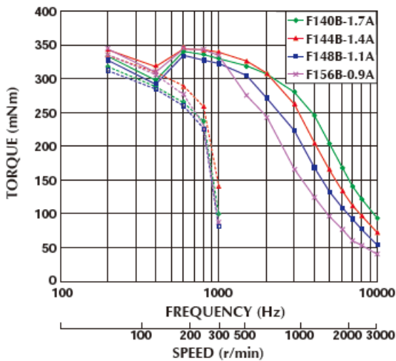
Model No: 17PM-F140B,F144B,F148B,F156B Driver: Chopper Dual Supply Voltage: 24.0 (Volt)
