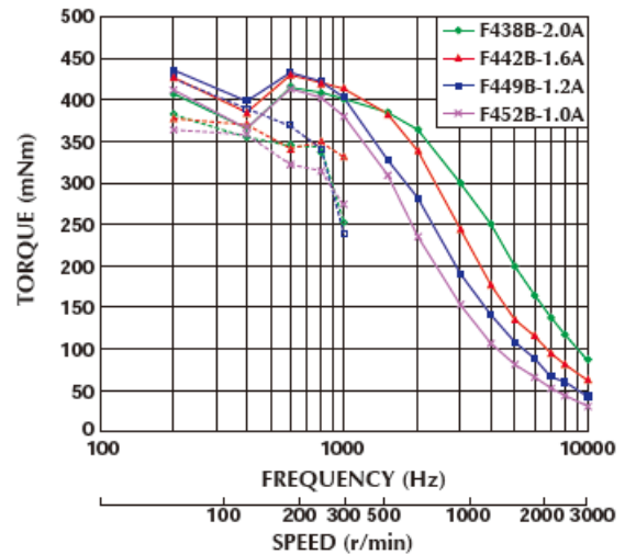
Model No: 17PM-FA38B,FA49B Driver: Chopper Dual Supply Voltage: 24.0 (Volt)
