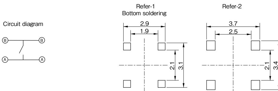
Reference land dimensions
