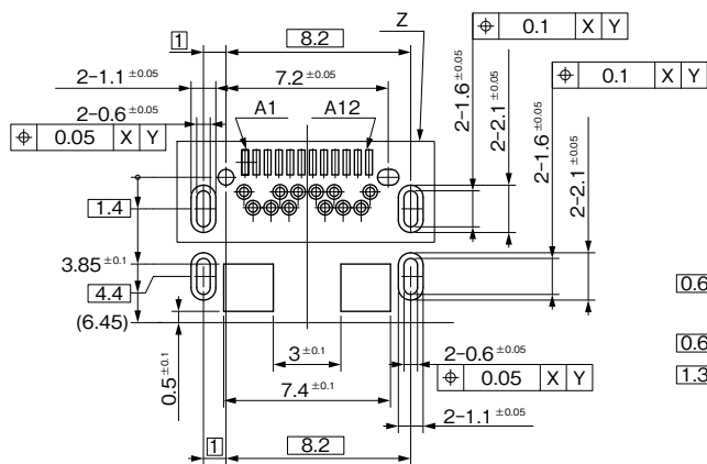
RECOMMENDED PWB LAYOUT (REFERENCE)
