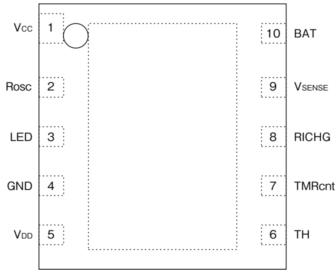
PLP-10 (TOP VIEW)
