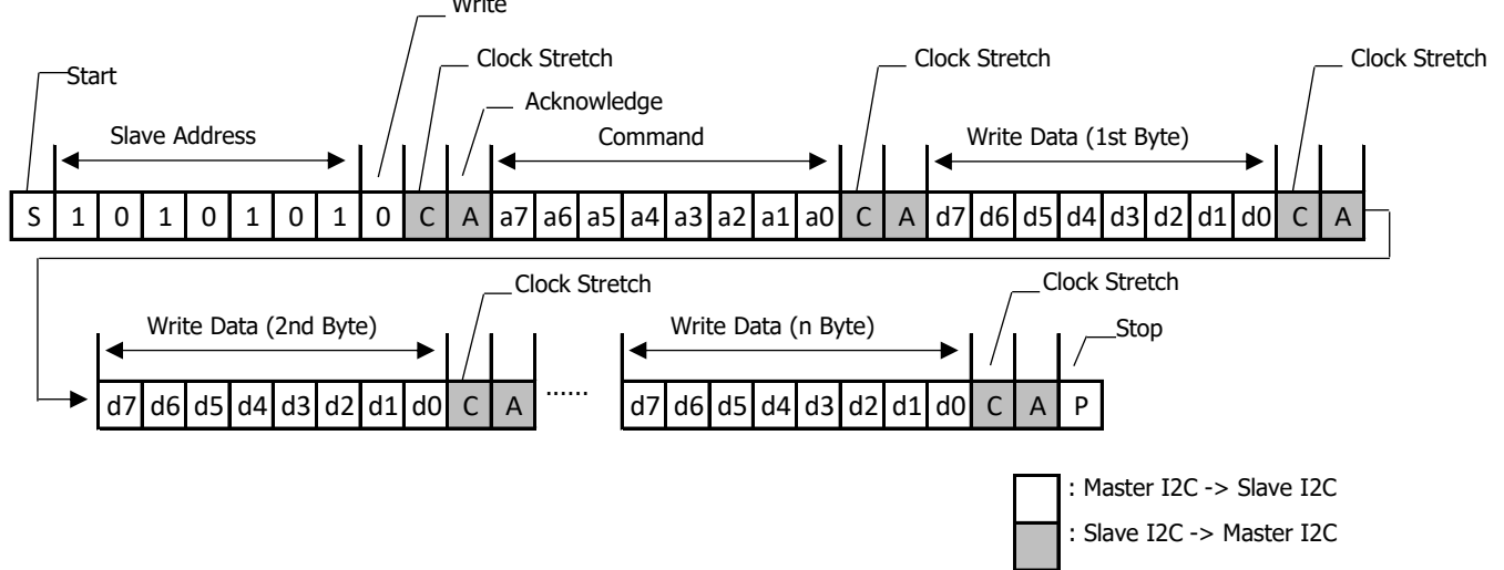
I2C read format (1 byte read : Device → Host)
